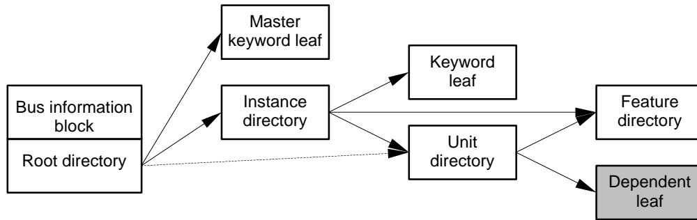
Figure 15 – Example configuration ROM hierarchy
