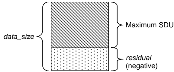
Figure 19 – Excess initiator data (datagram model)
