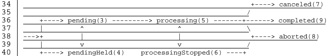
41 42 Figure 1 - Normal Job State Transitions
