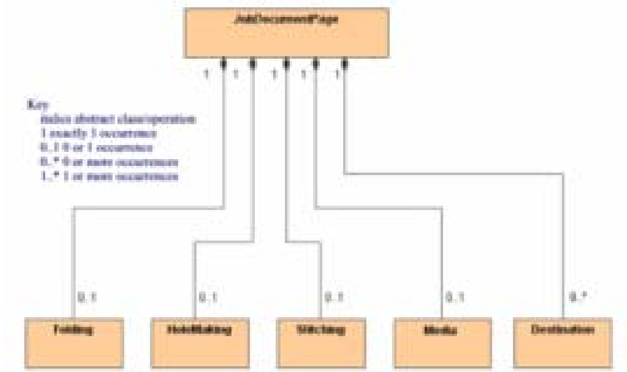
Figure 2.0 JTAPI JobDocumentPage High Level Object Model
